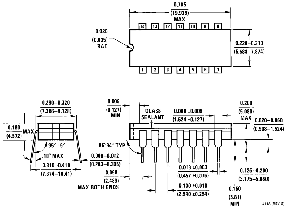
Cavity Dual-In Line Package (J) Order Number MM54HC04J or MM74HC04J See NS Package J14A
